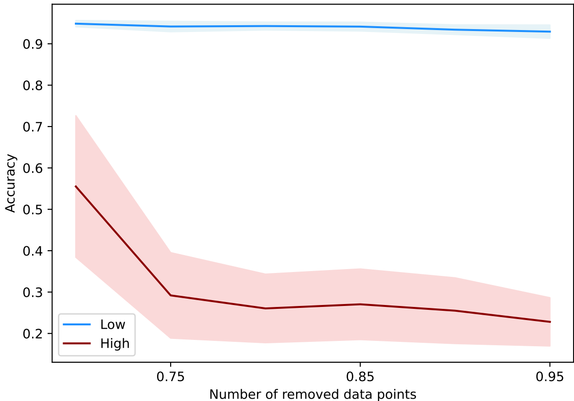
DataAttrOpt(10000, 0.05, 15, best, +b, alpha=best) - bbc-embeddings
